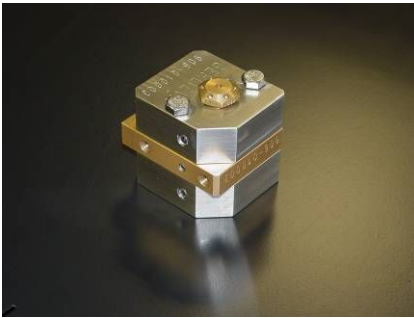
2-circuit custom designed sprayhead for 1 spraying media
